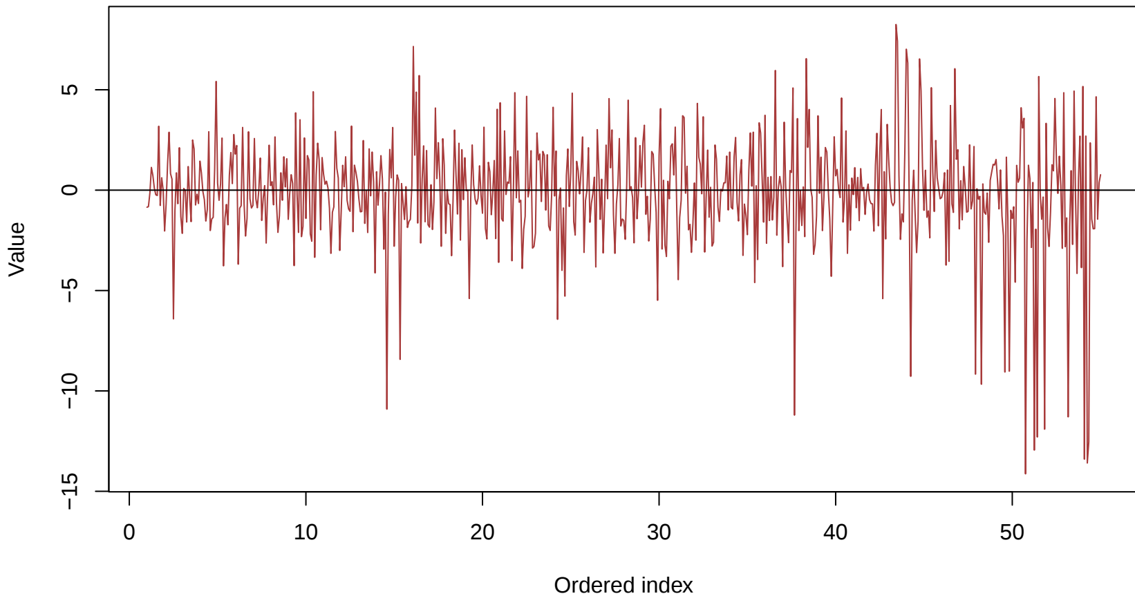
Time Series in R residual or transformed series
