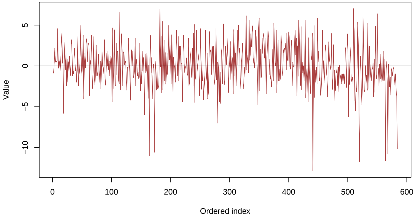
Time Series in Python residual or transformed series
