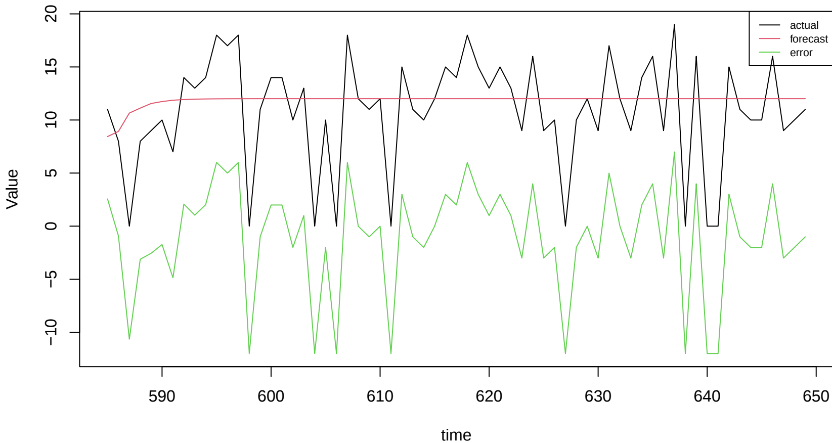
Time Series in Python method-specific output
