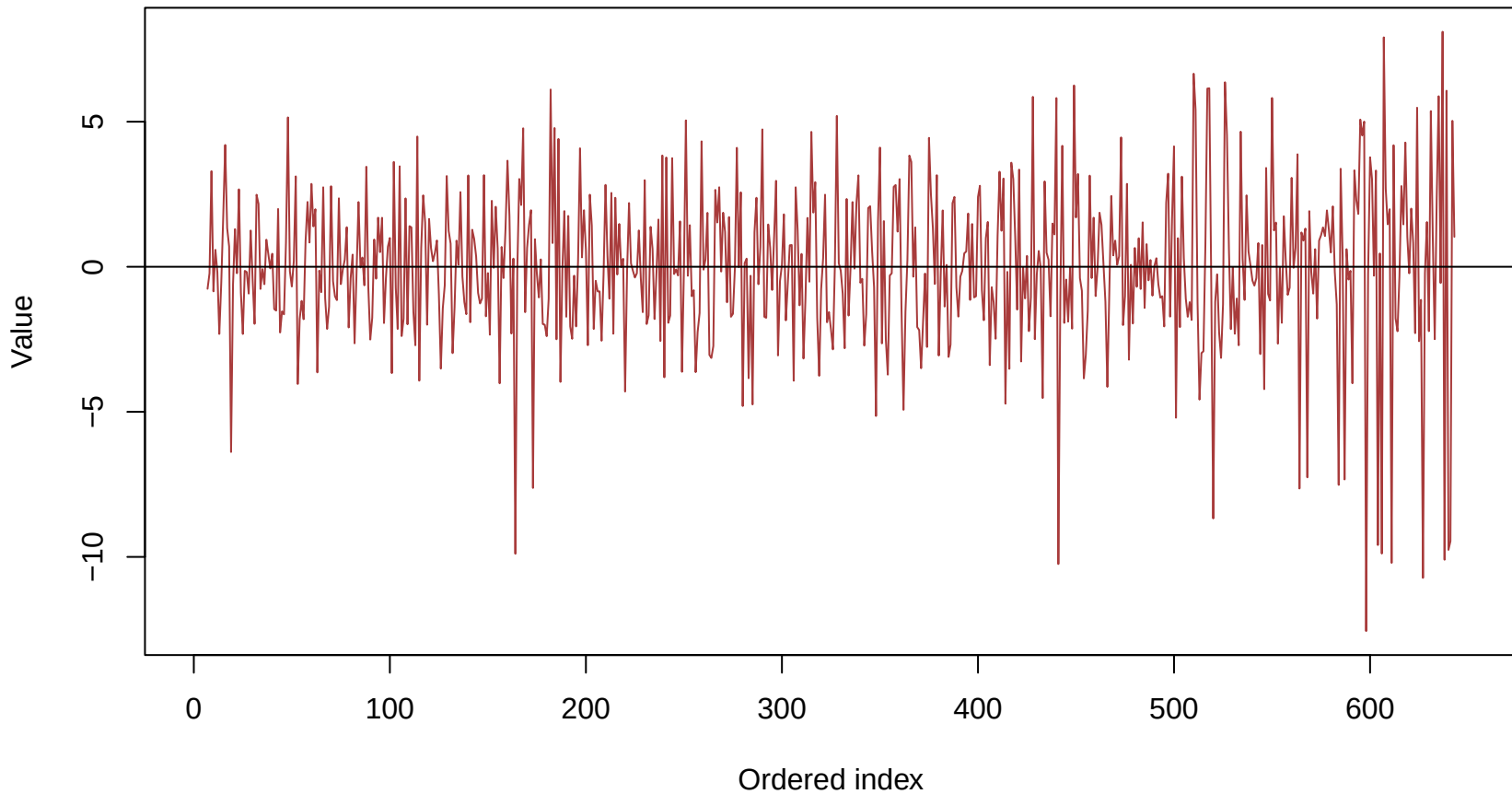
Seasonal Decomposition residual or transformed series
