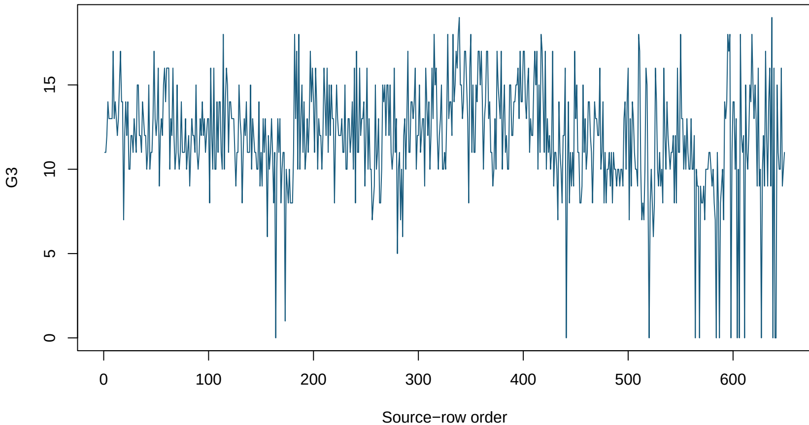
Seasonal Decomposition source-row ordered G3
