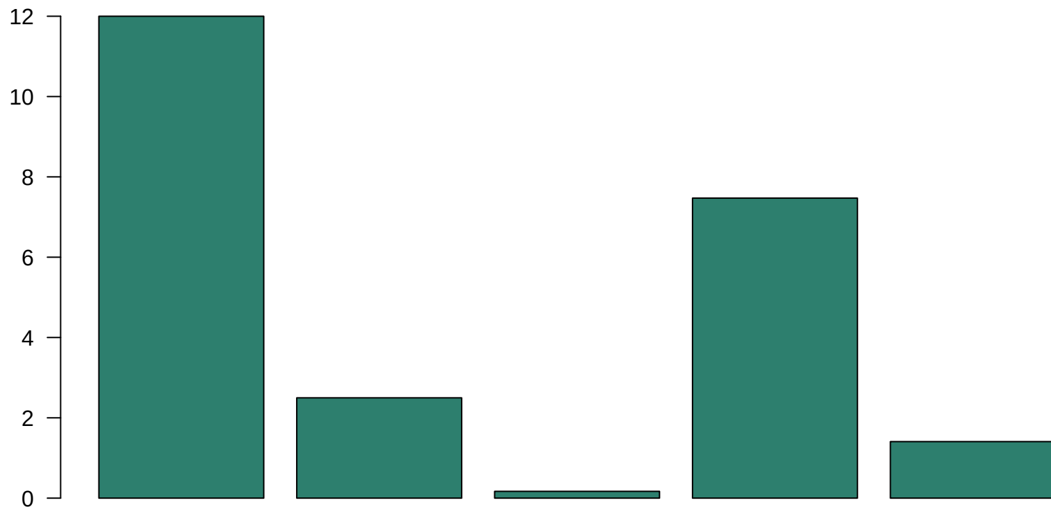
Seasonal Decomposition primary metrics
