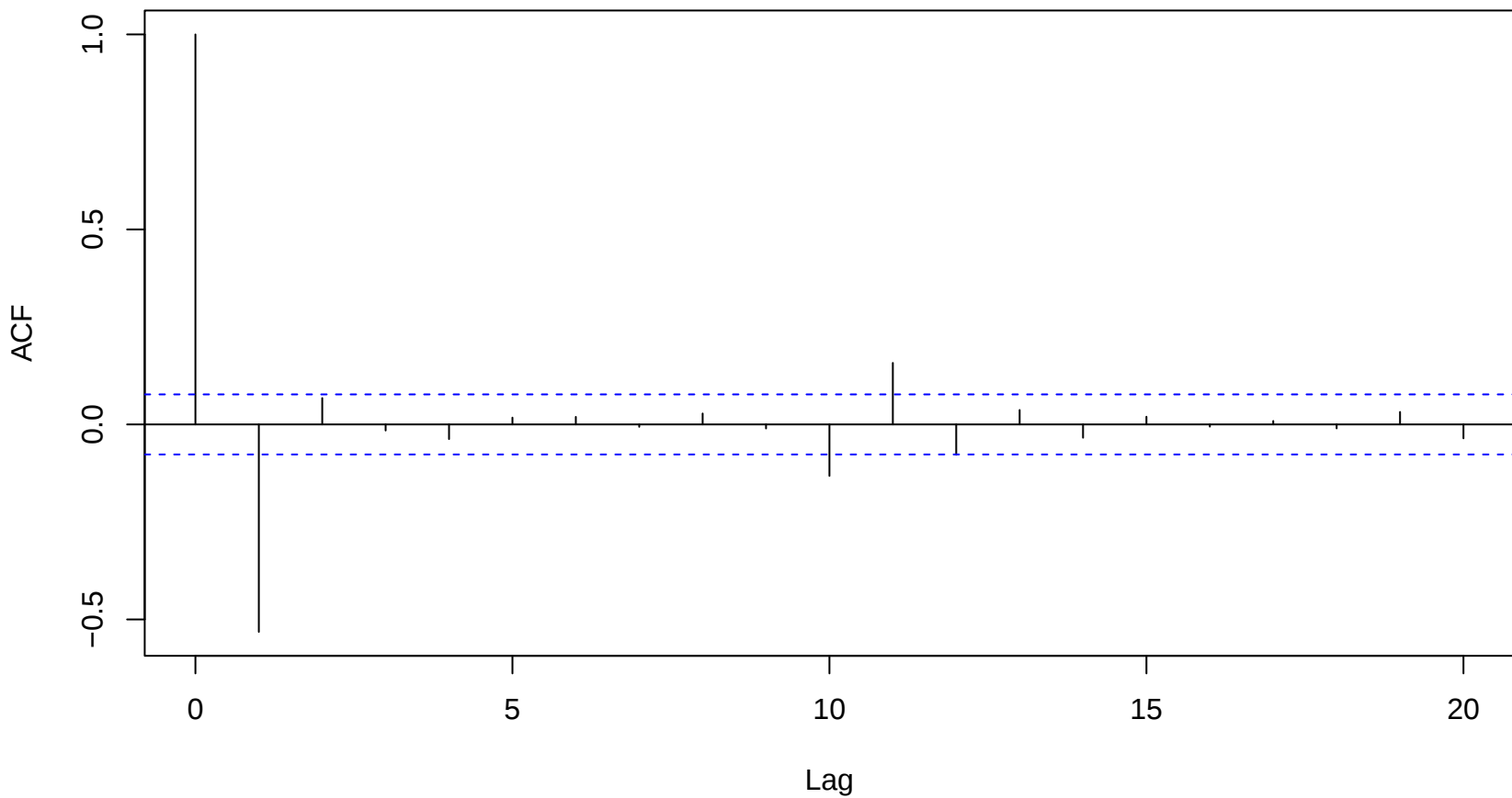
RMSE residual dependence
