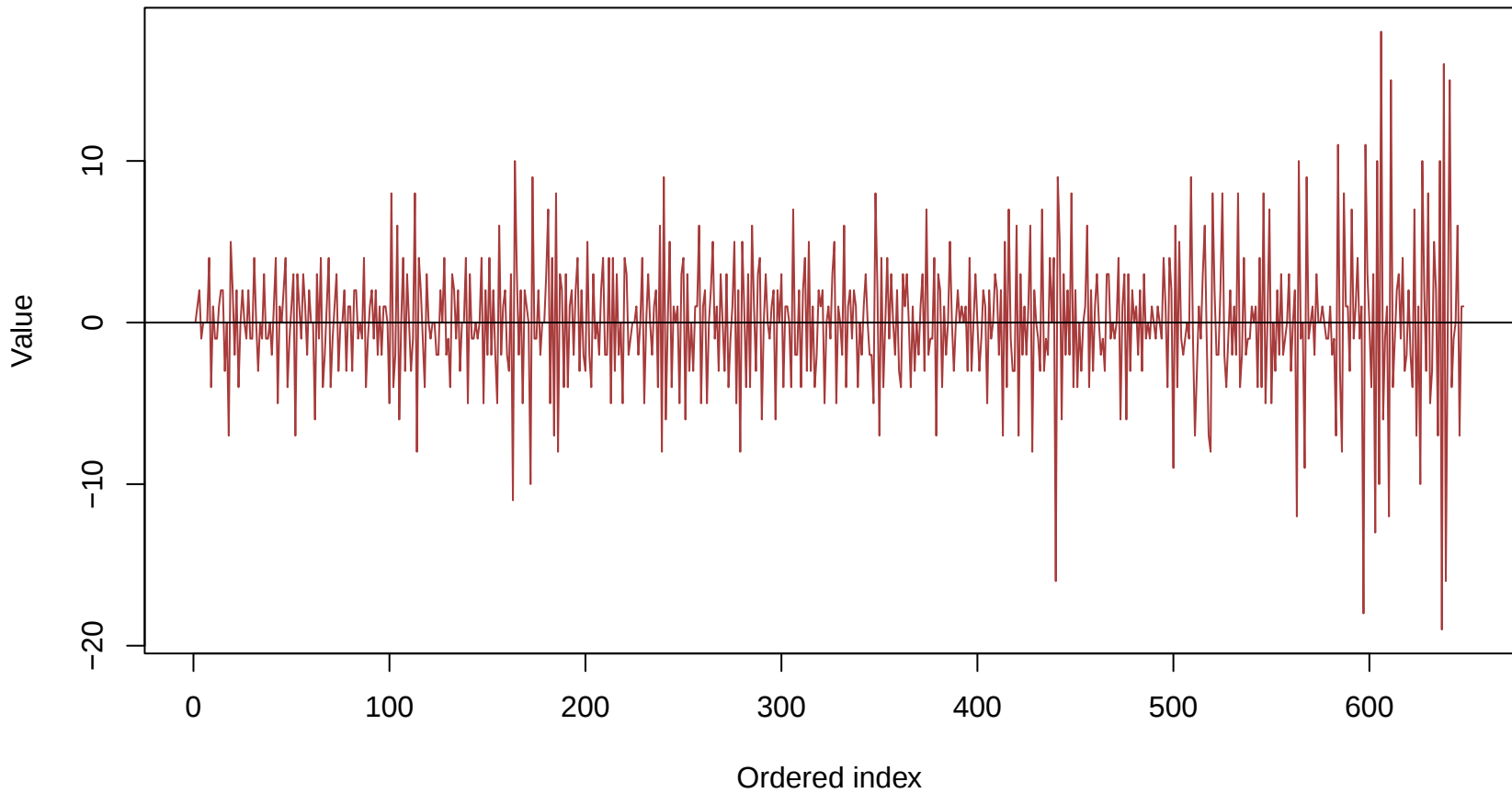
RMSE residual or transformed series
