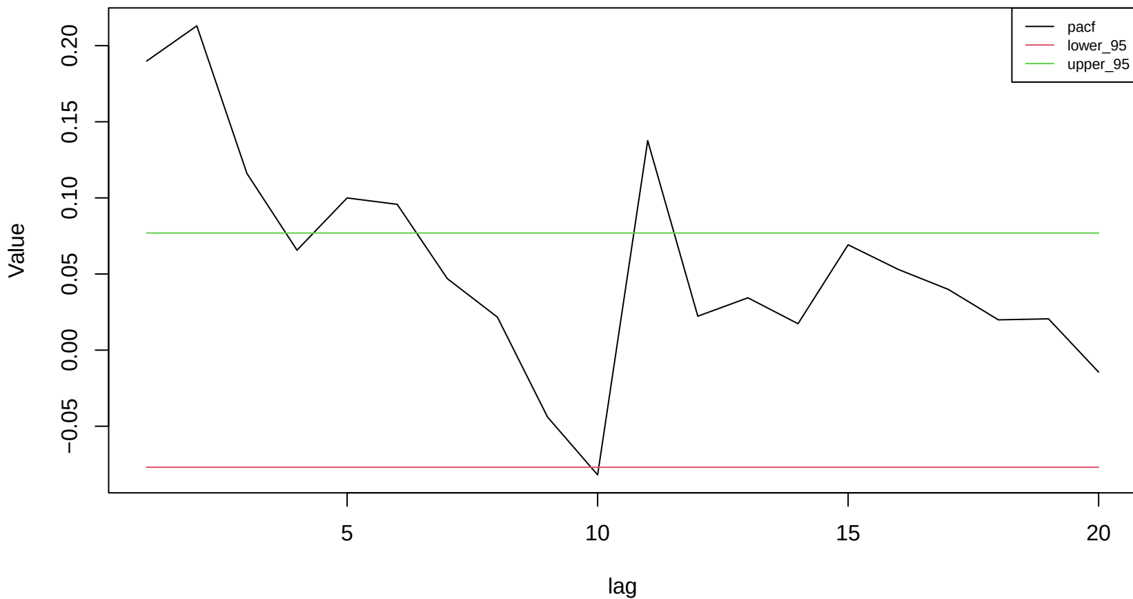
Partial Autocorrelation Function method-specific output
