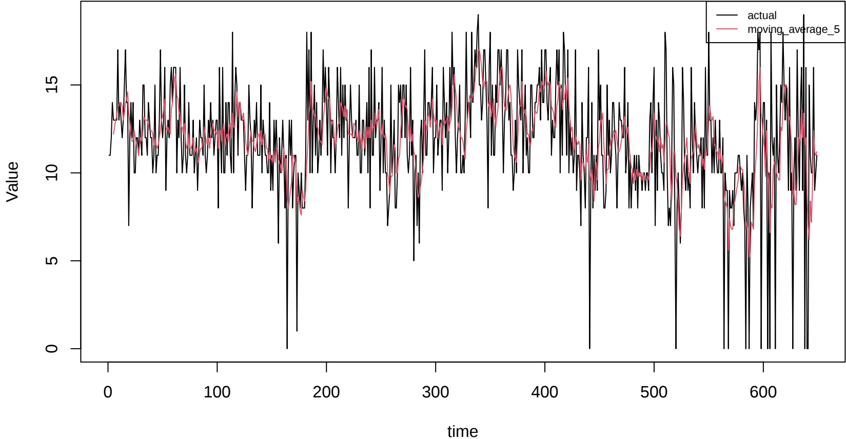
Moving Average method-specific output
