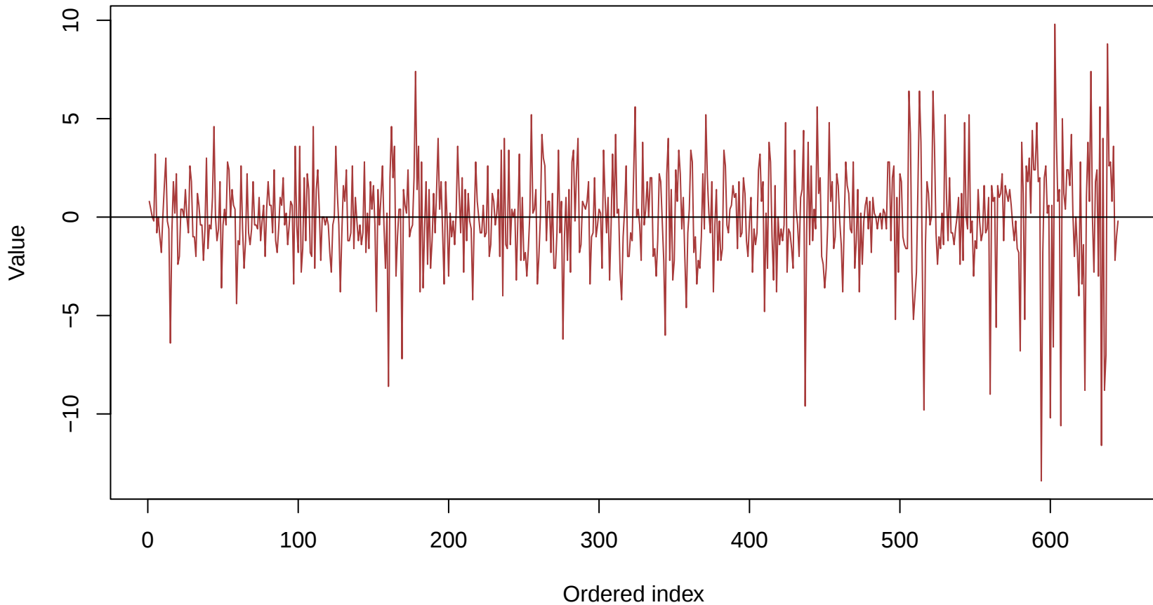
Moving Average residual or transformed series
