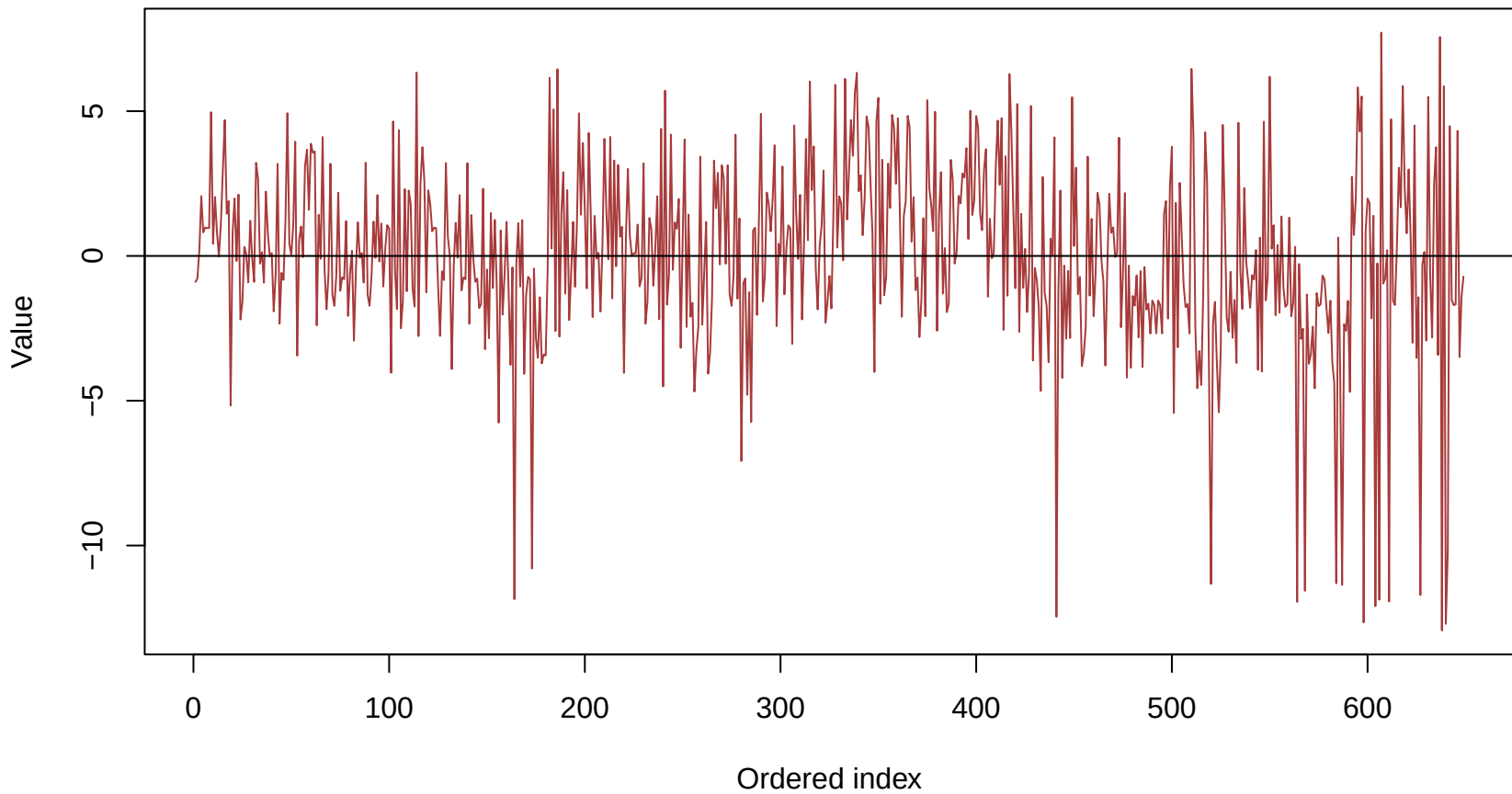
MA Model residual or transformed series
