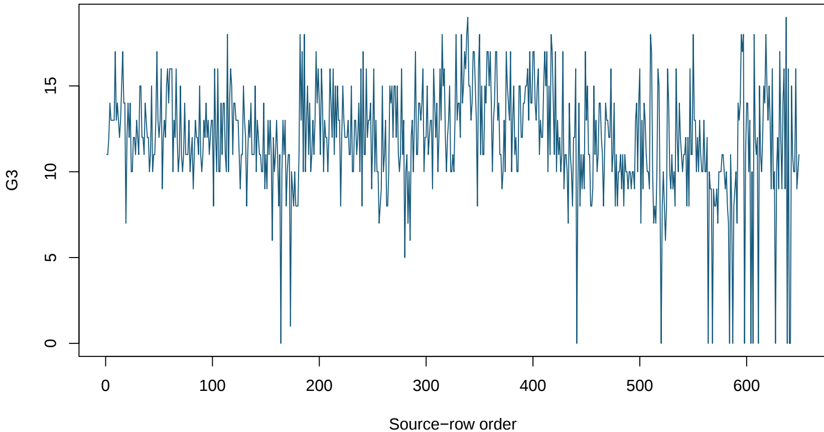
Holts Linear Trend Method source-row ordered G3
