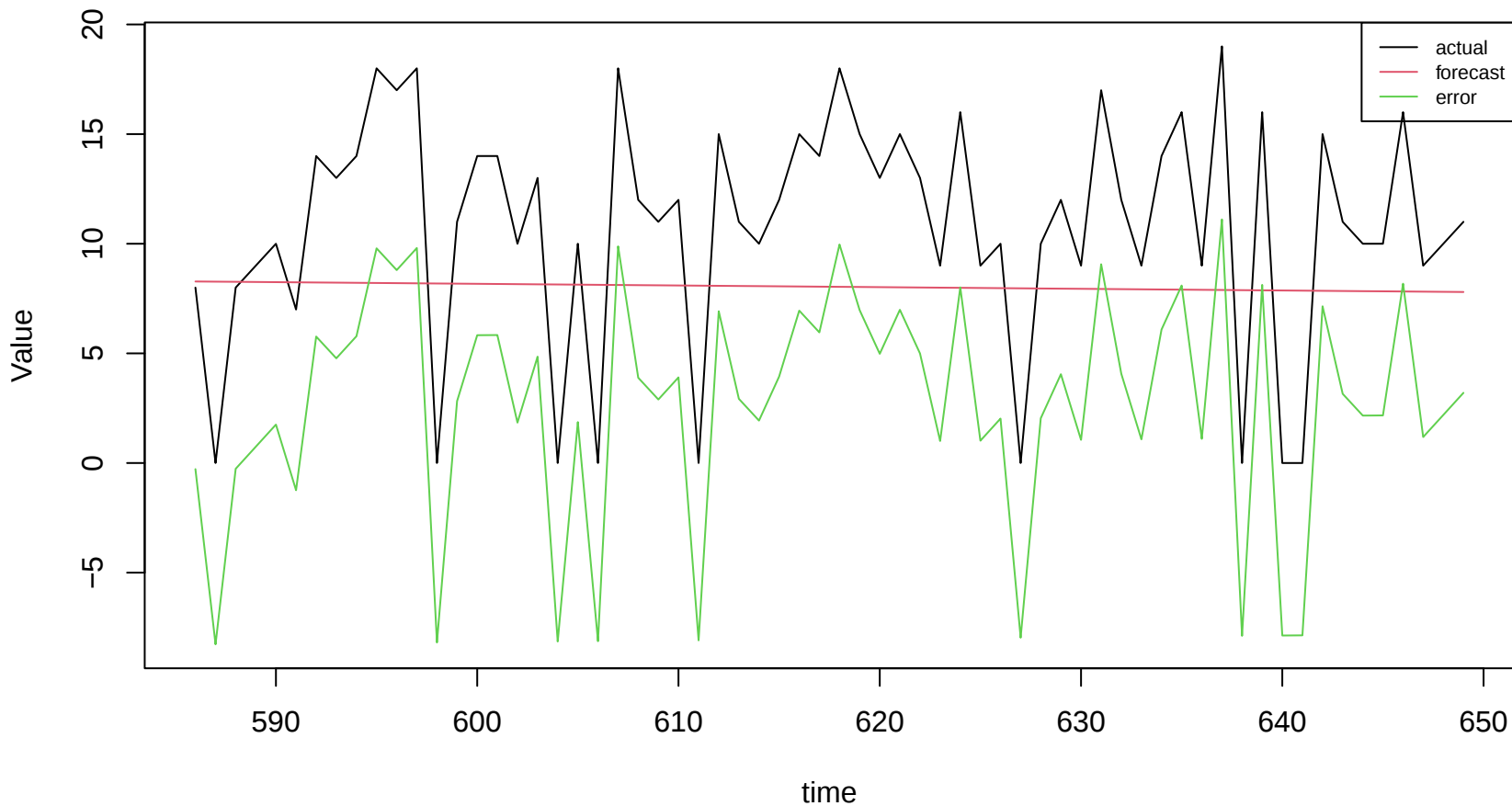
Holts Linear Trend Method method-specific output
