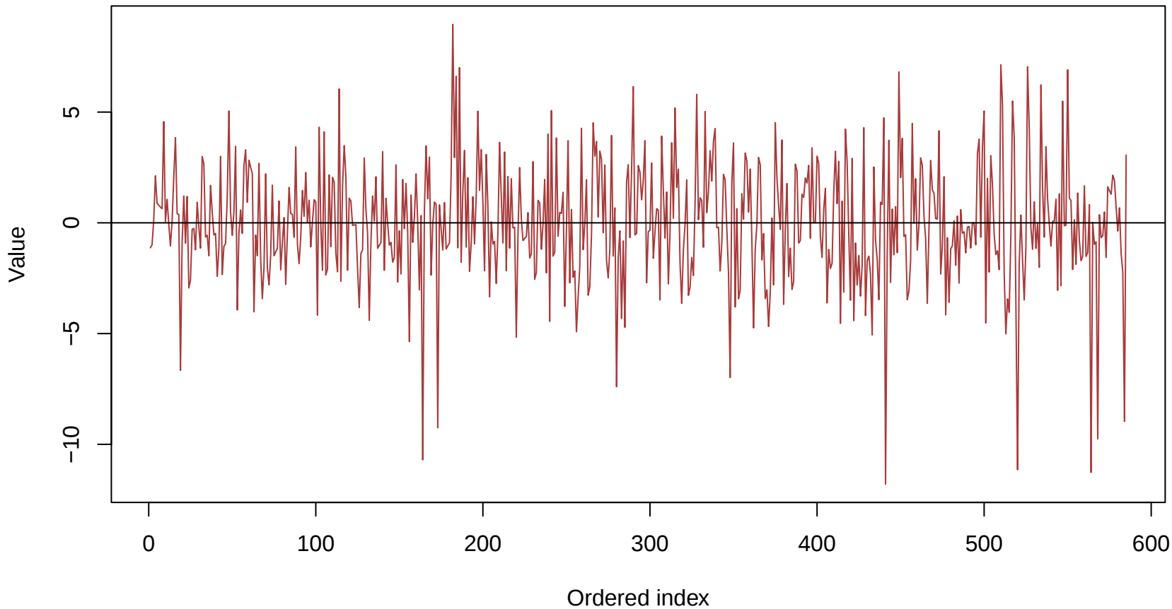
Holts Linear Trend Method residual or transformed series
