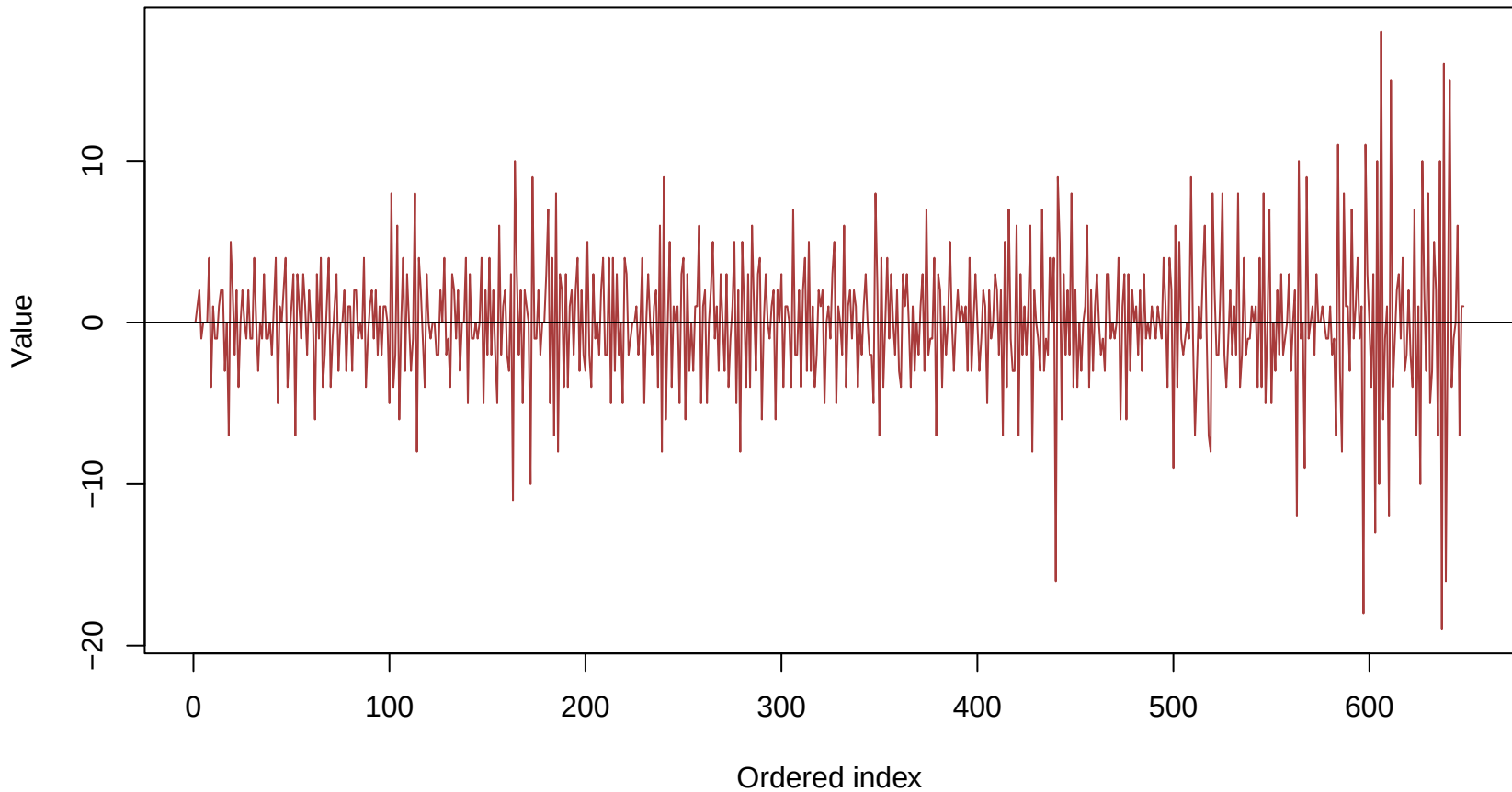
Forecast Accuracy Metrics residual or transformed series
