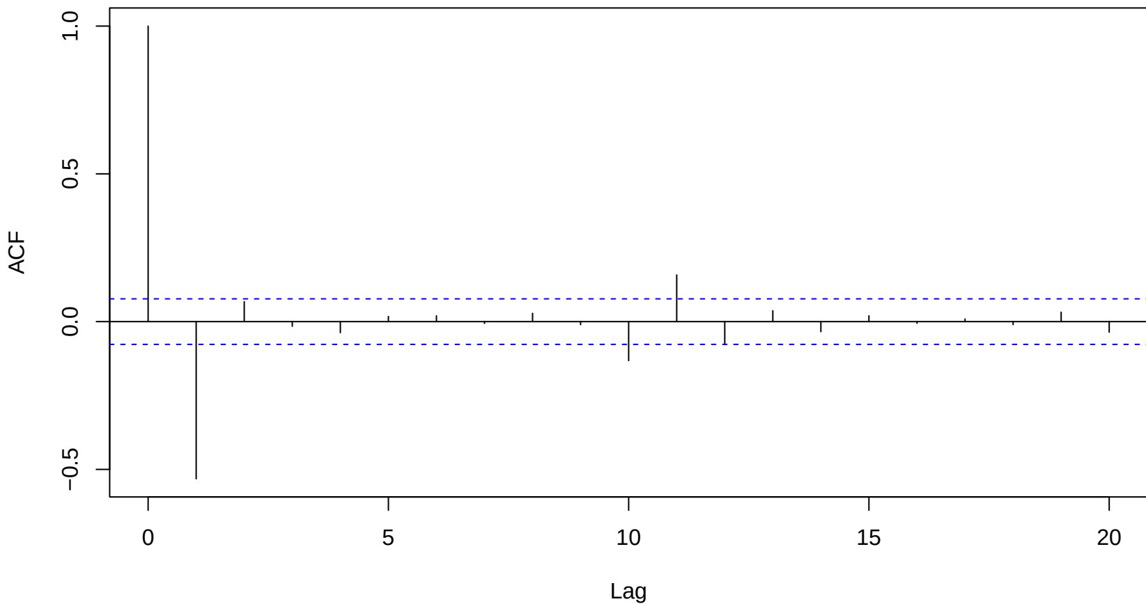
Forecast Accuracy Metrics residual dependence
