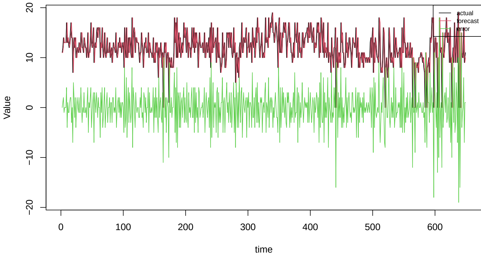
Forecast Accuracy Metrics method-specific output
