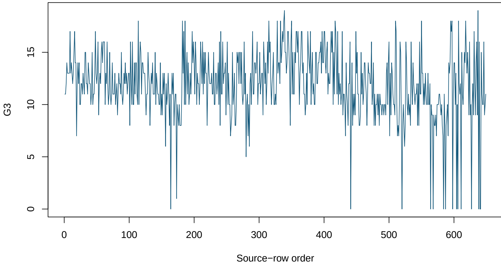
Forecast Accuracy Metrics source-row ordered G3
