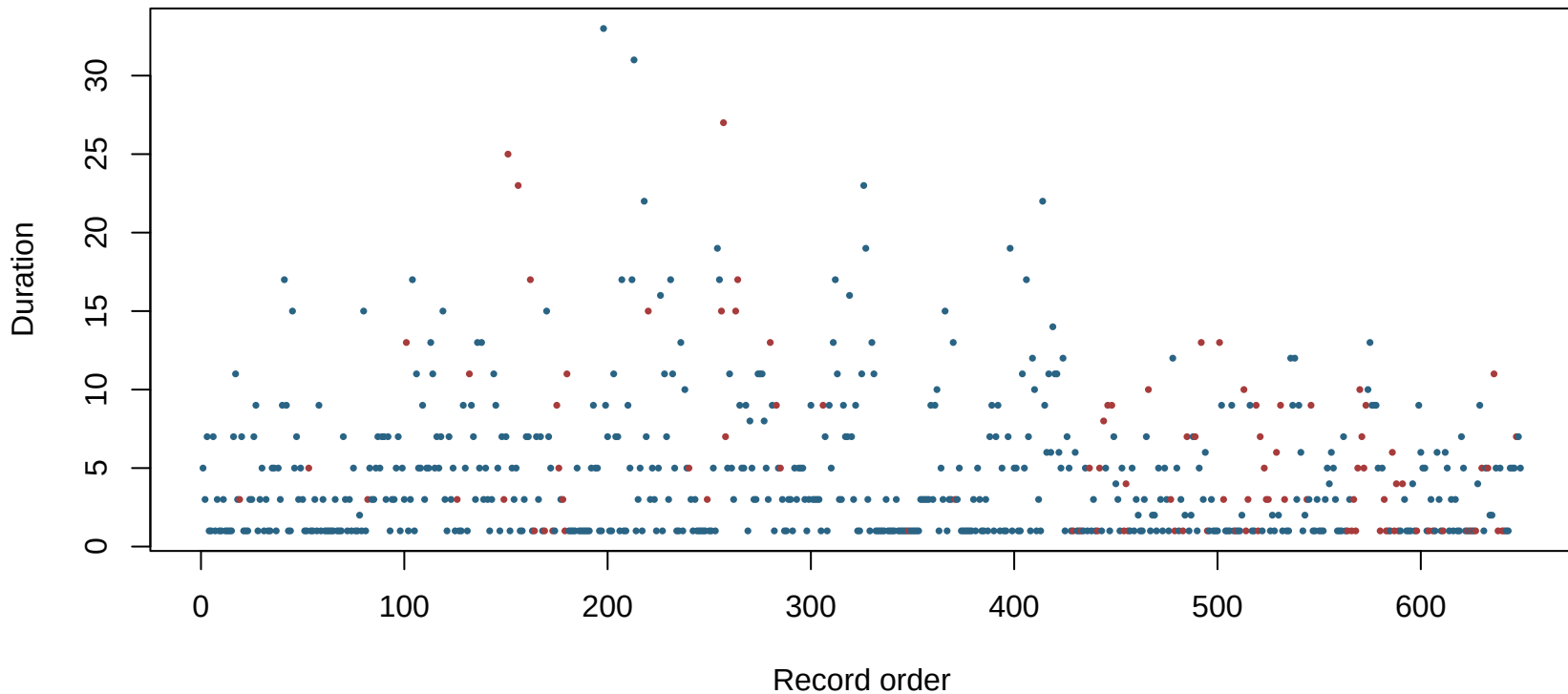
Fine Gray Model encoded follow-up
