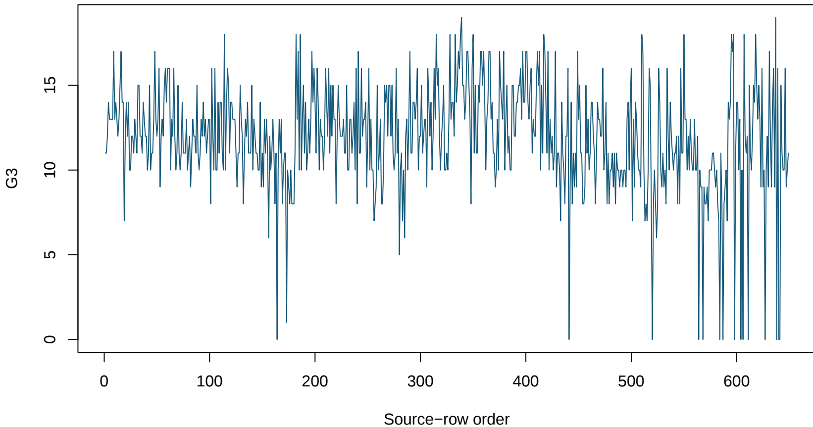
Chow Test source-row ordered G3
