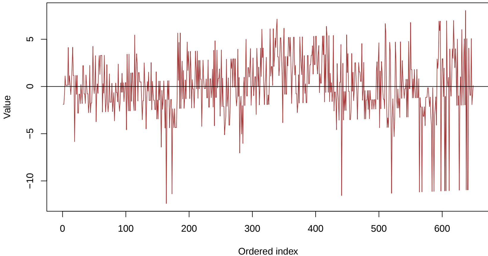
Chow Test residual or transformed series
