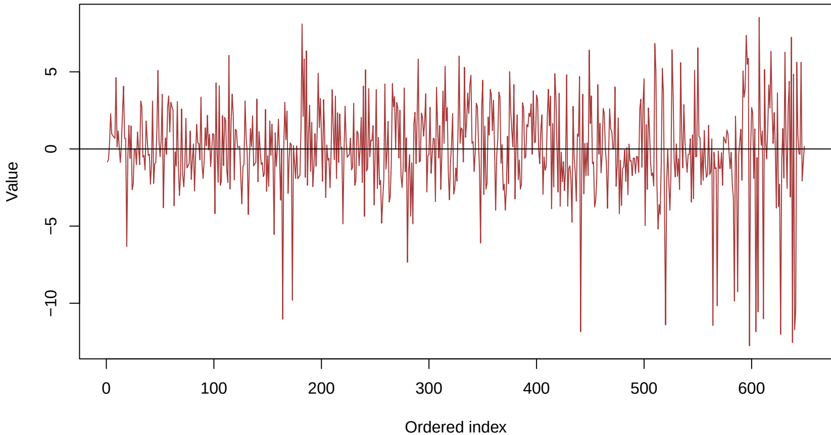
ARMA Model residual or transformed series
