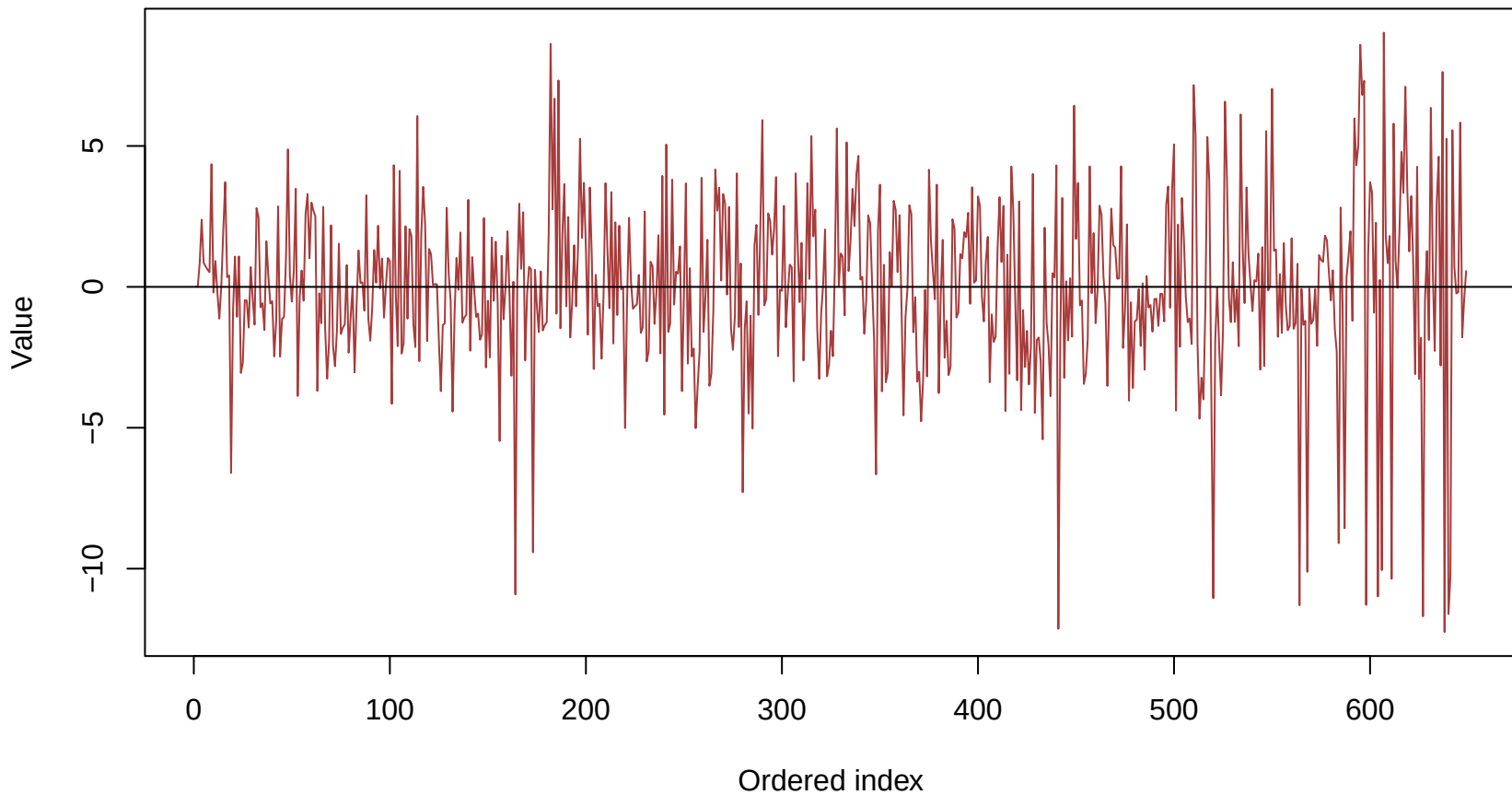
ARIMA Model residual or transformed series
