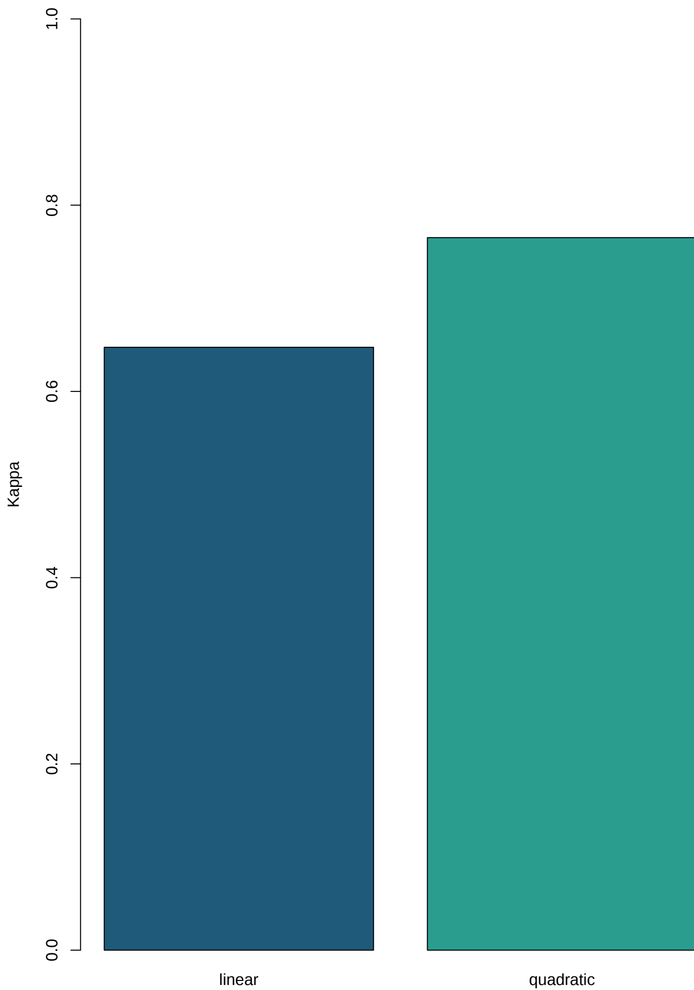
Linear and quadratic weighted kappa
