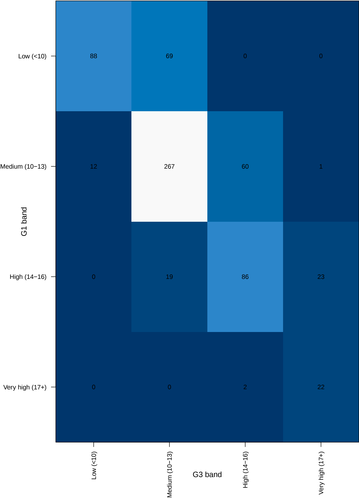
Ordinal G1-by-G3 agreement
