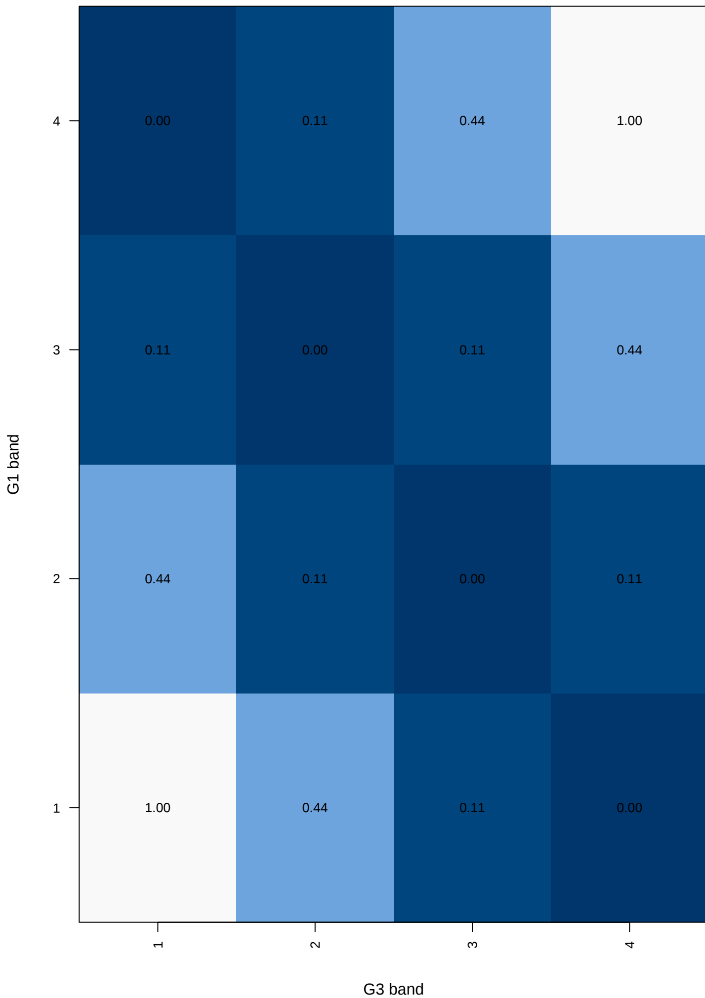
Quadratic disagreement weights
