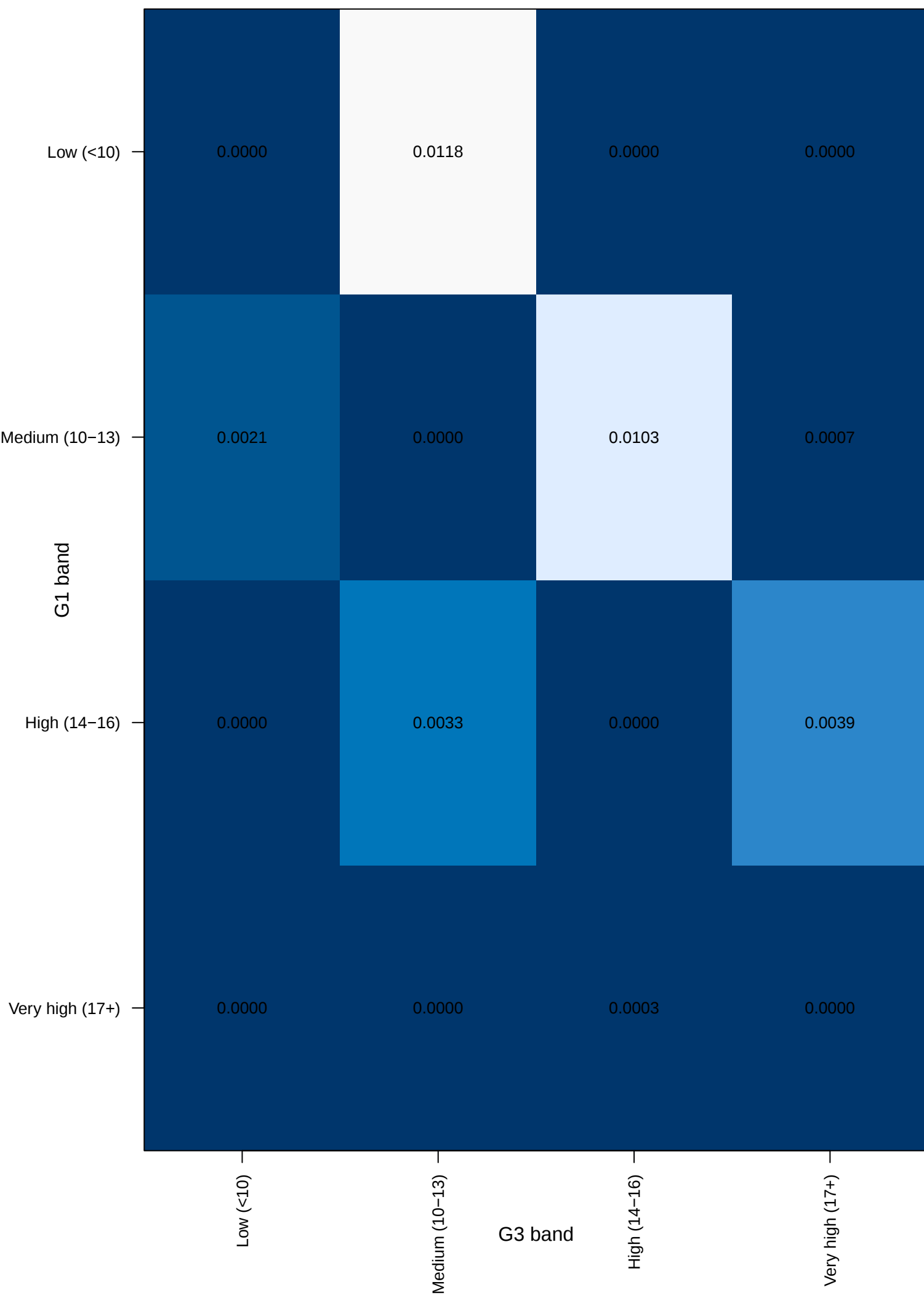
Observed quadratic disagreement contributions
