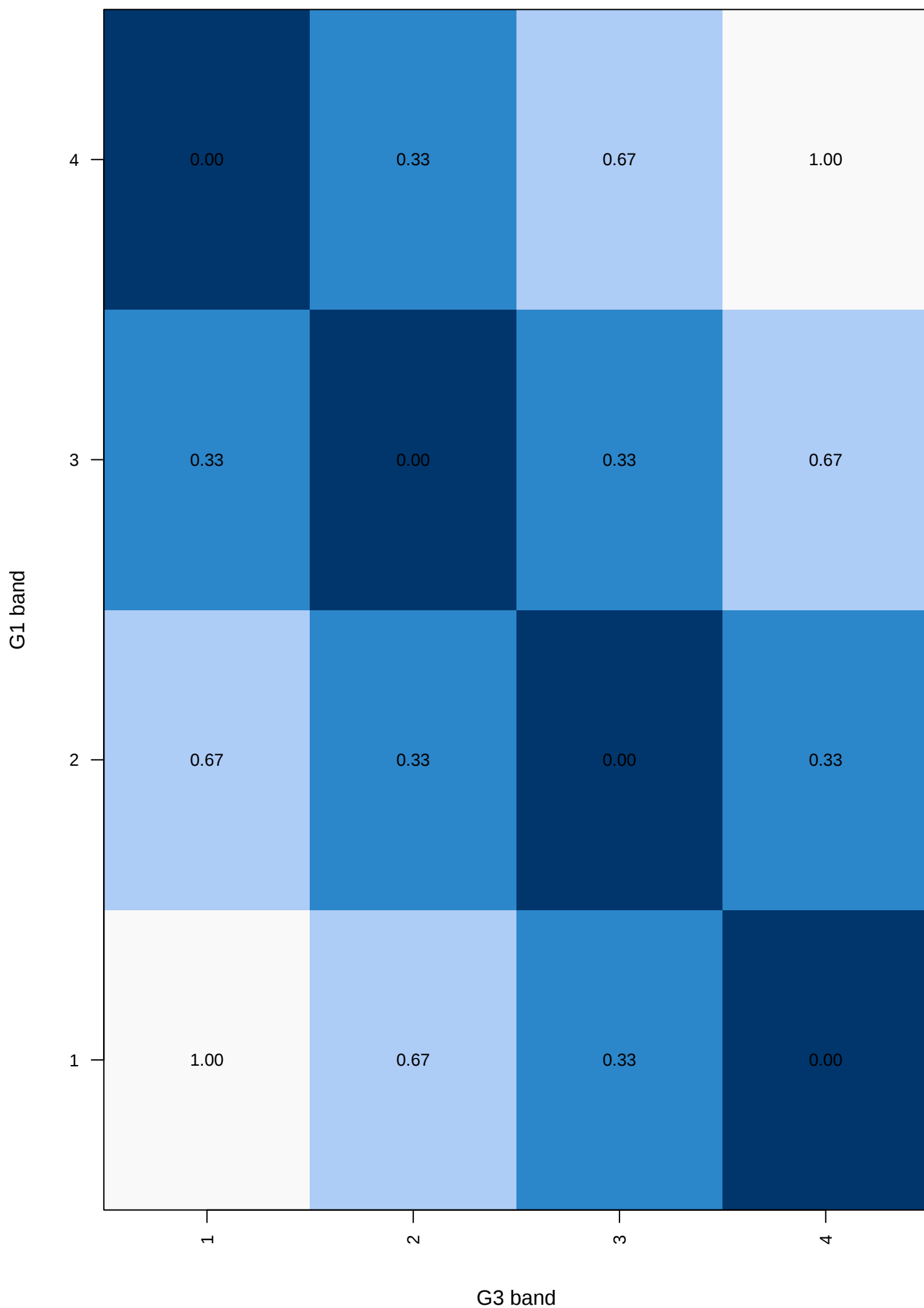
Linear disagreement weights
