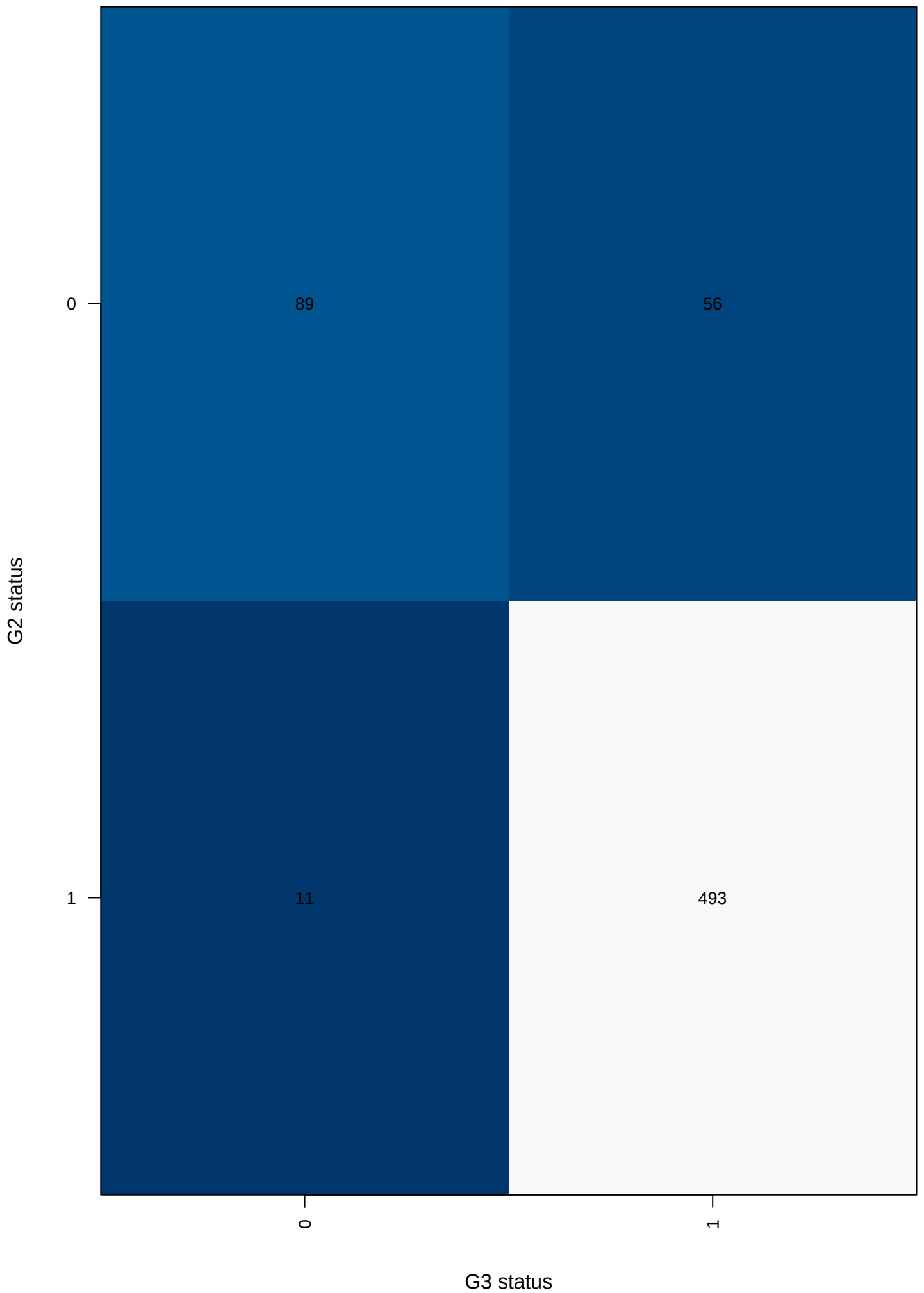
Paired G2/G3 pass transitions
