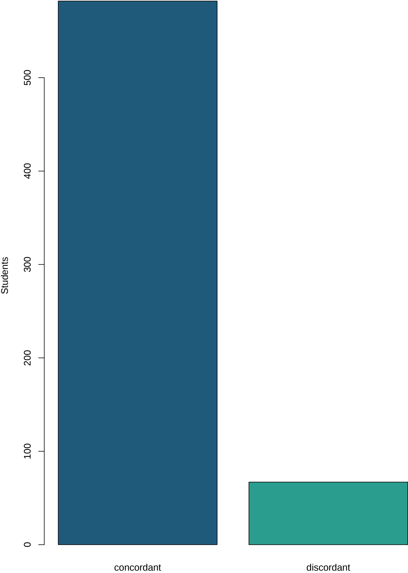
Concordant and discordant pairs
