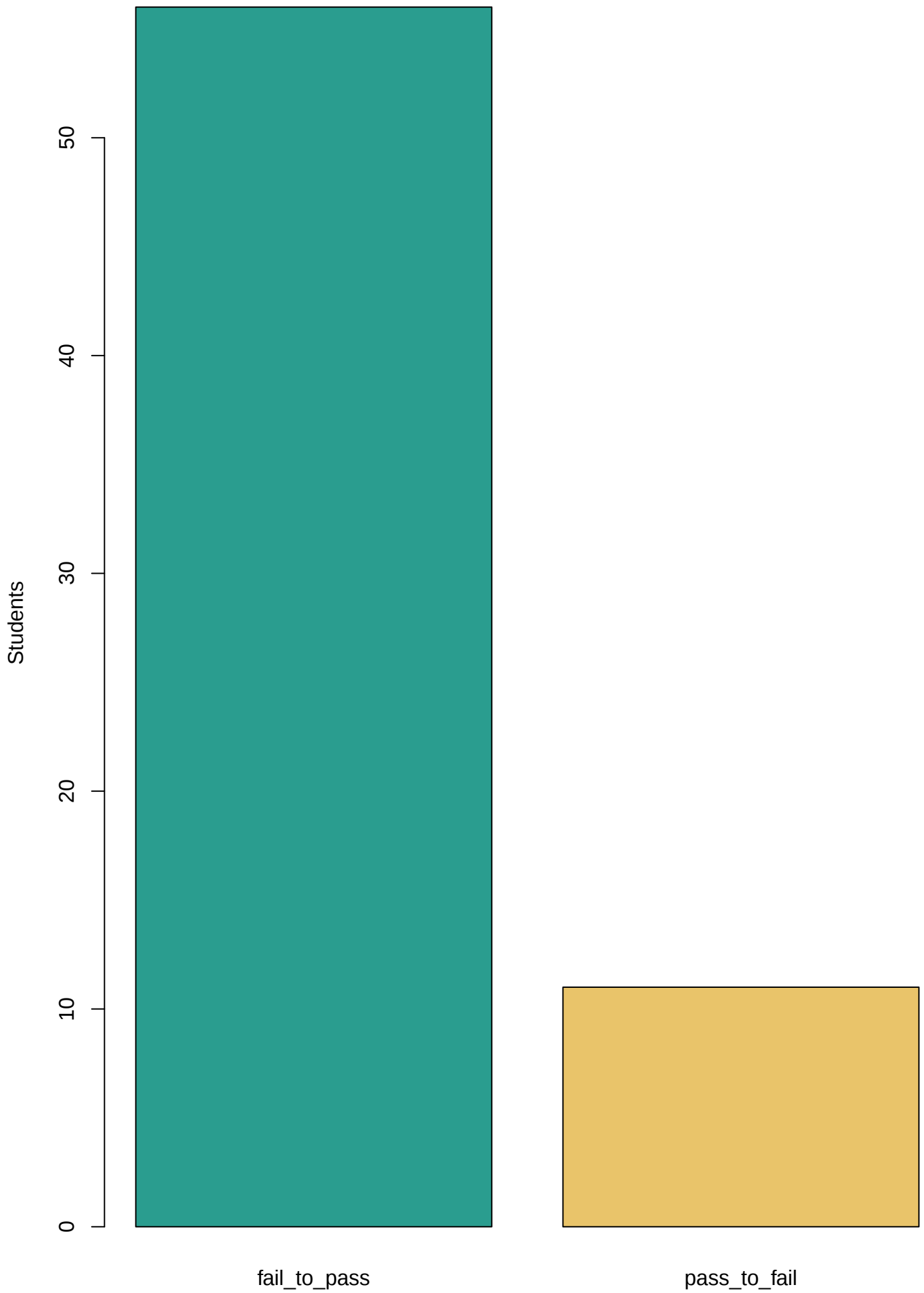
Discordant transition counts
