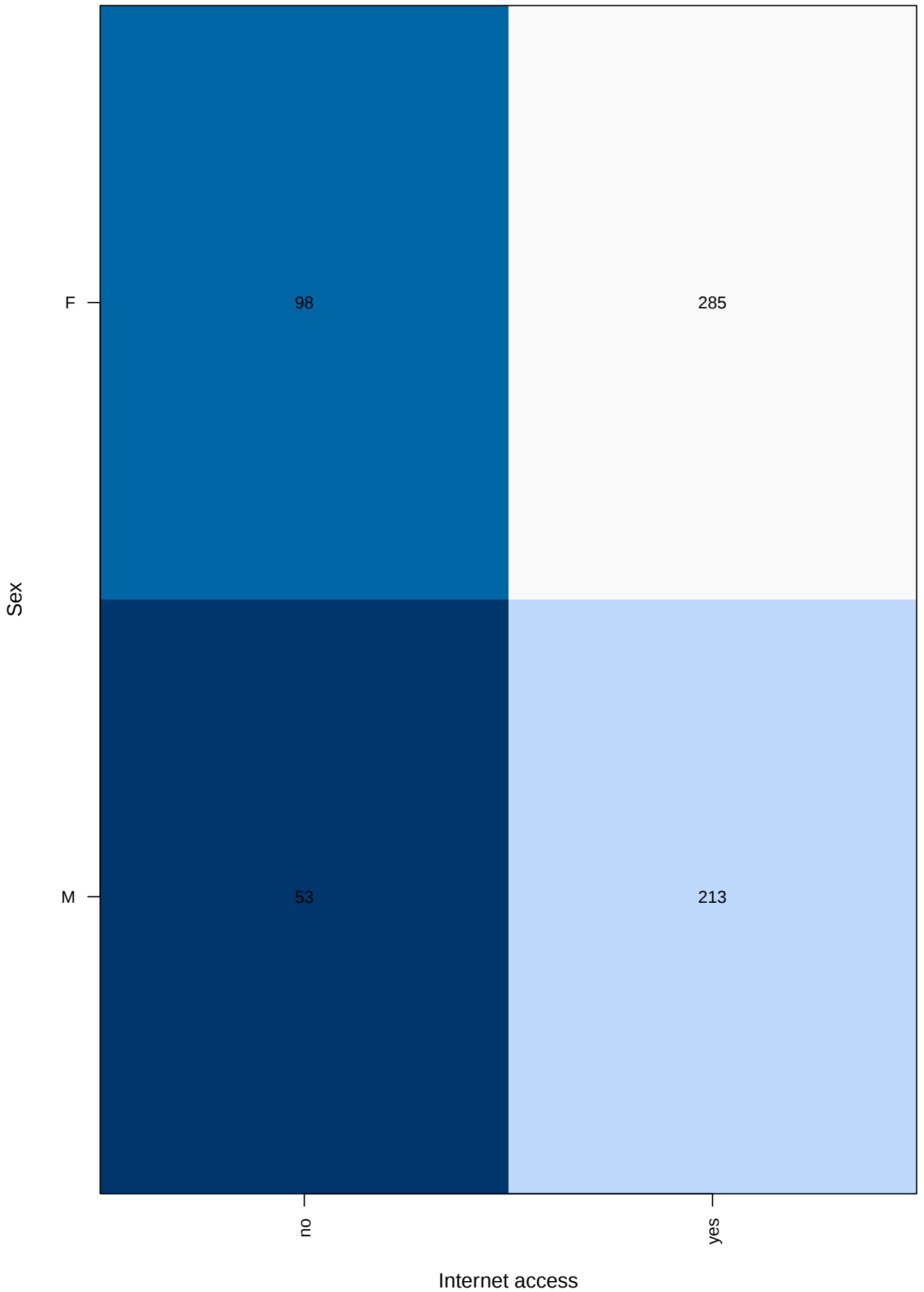
Sex by internet-access table
