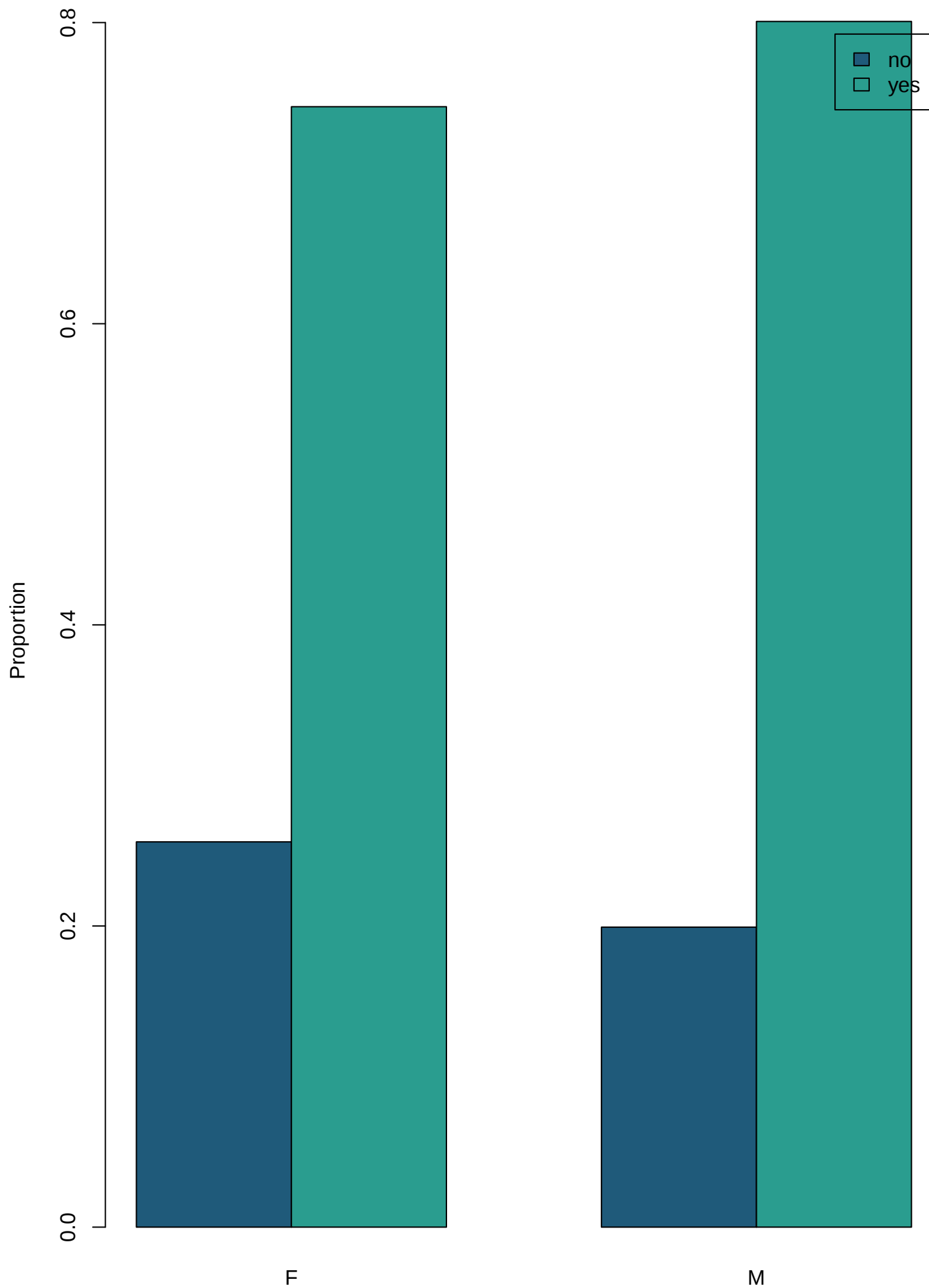
Internet access within sex
