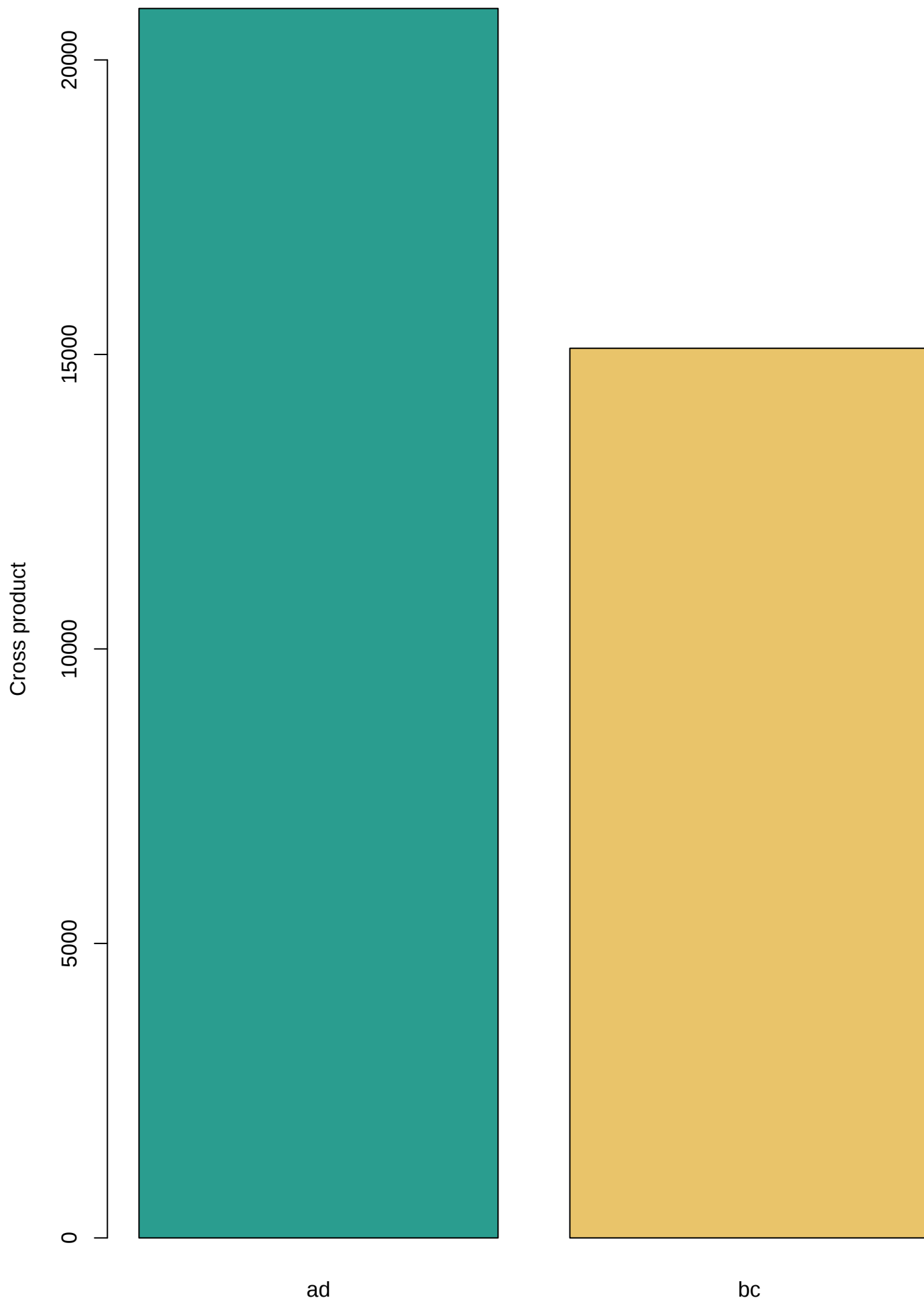
Cross-product components of sample odds ratio
