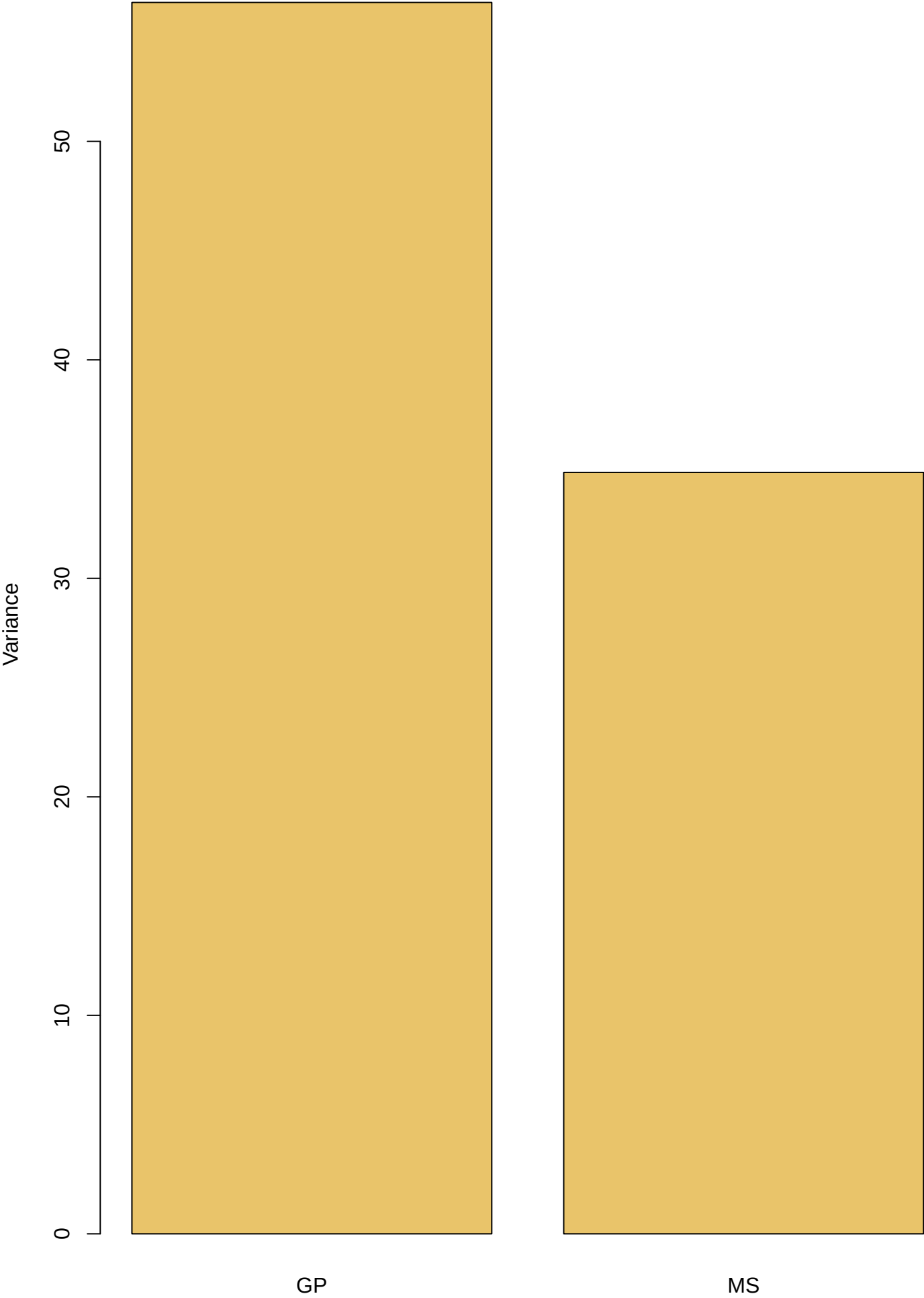
CMH variance by stratum
