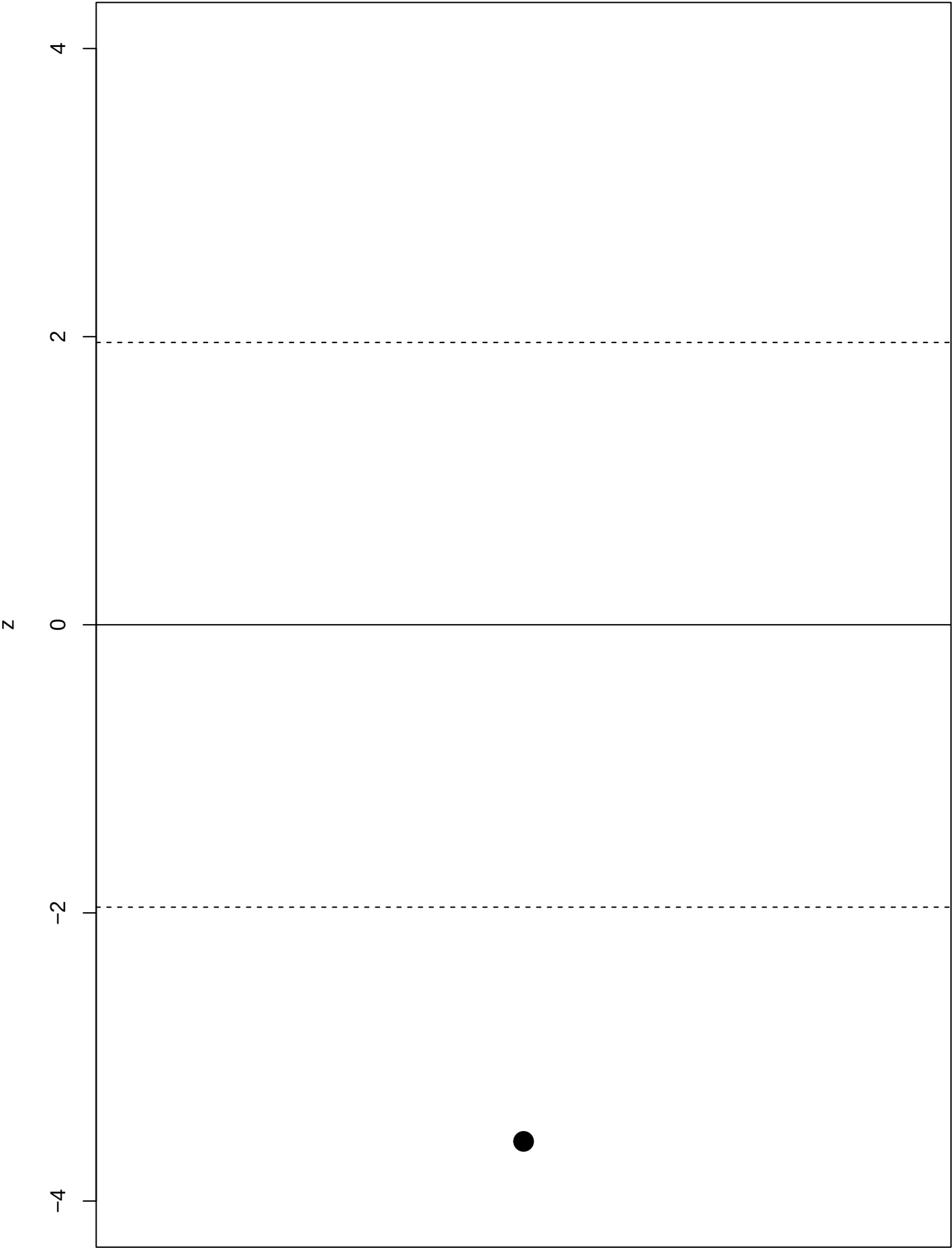
Signed CMH standard-normal score
