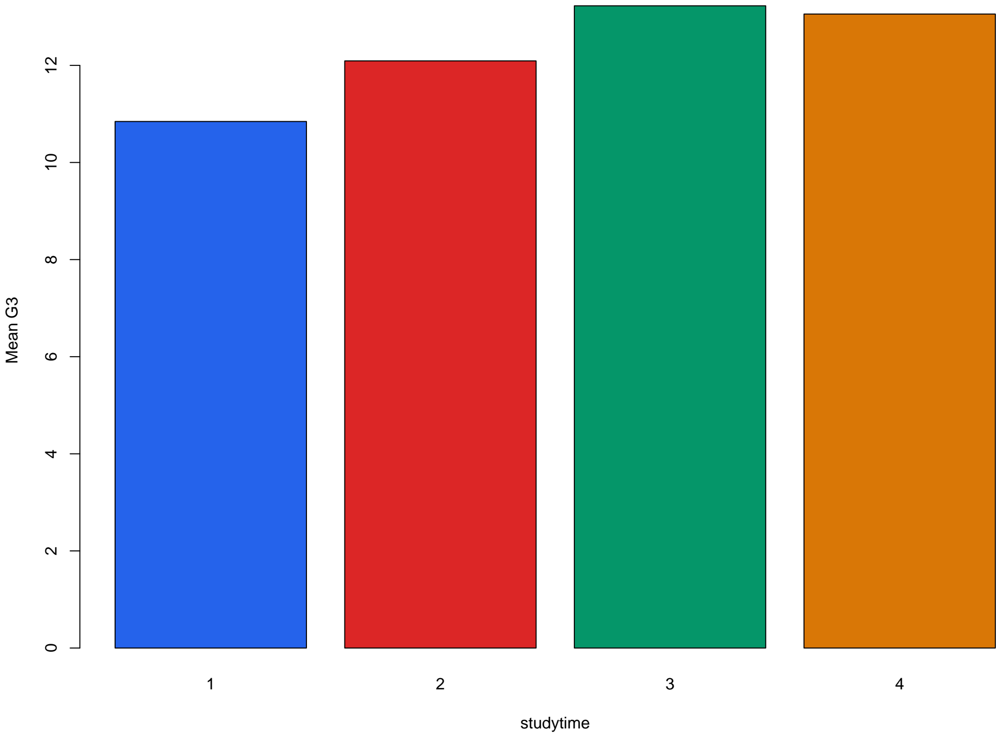
GLM ANOVA: Mean G3 by Studytime
