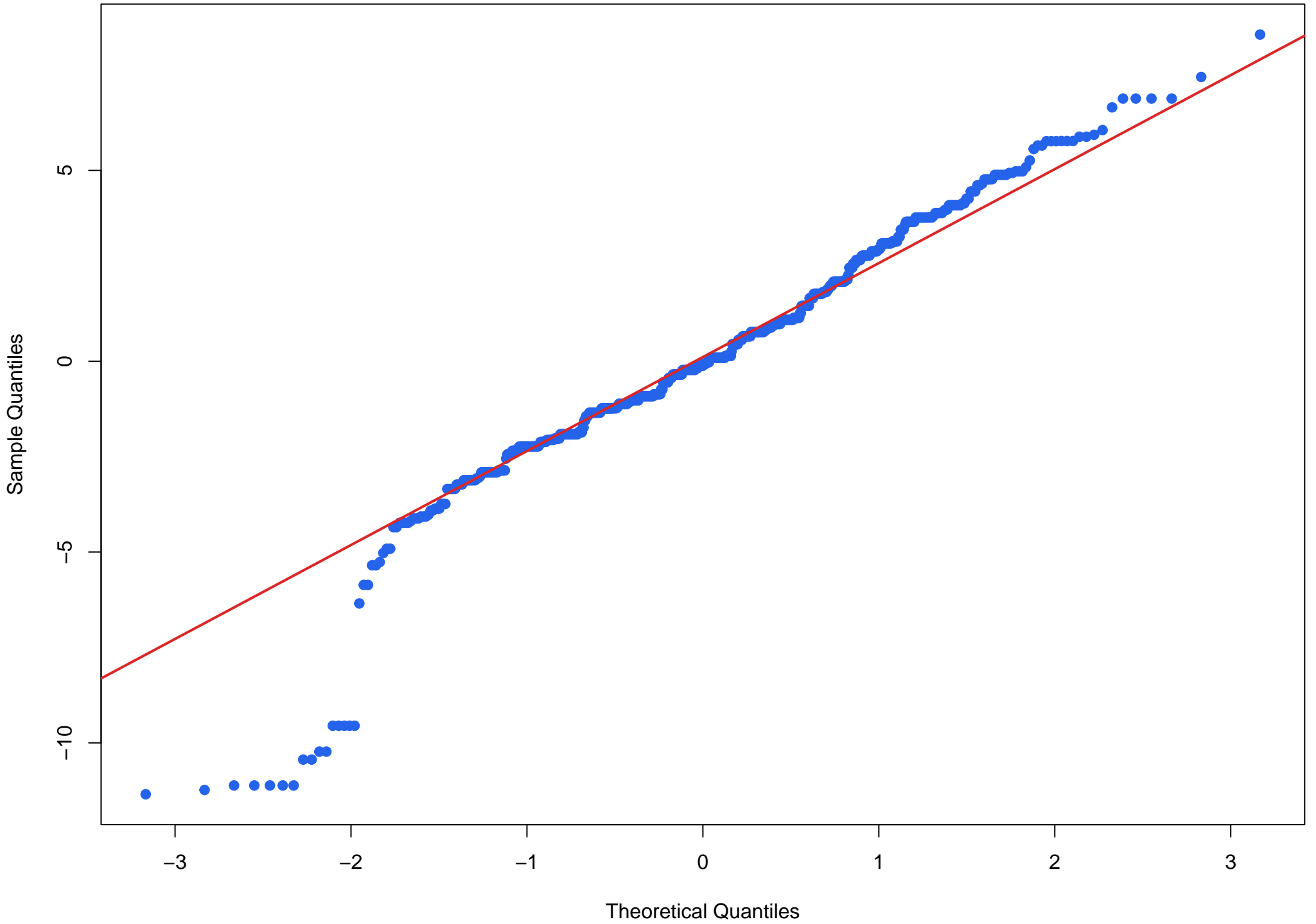
GLM ANOVA: Q-Q Plot of Residuals
