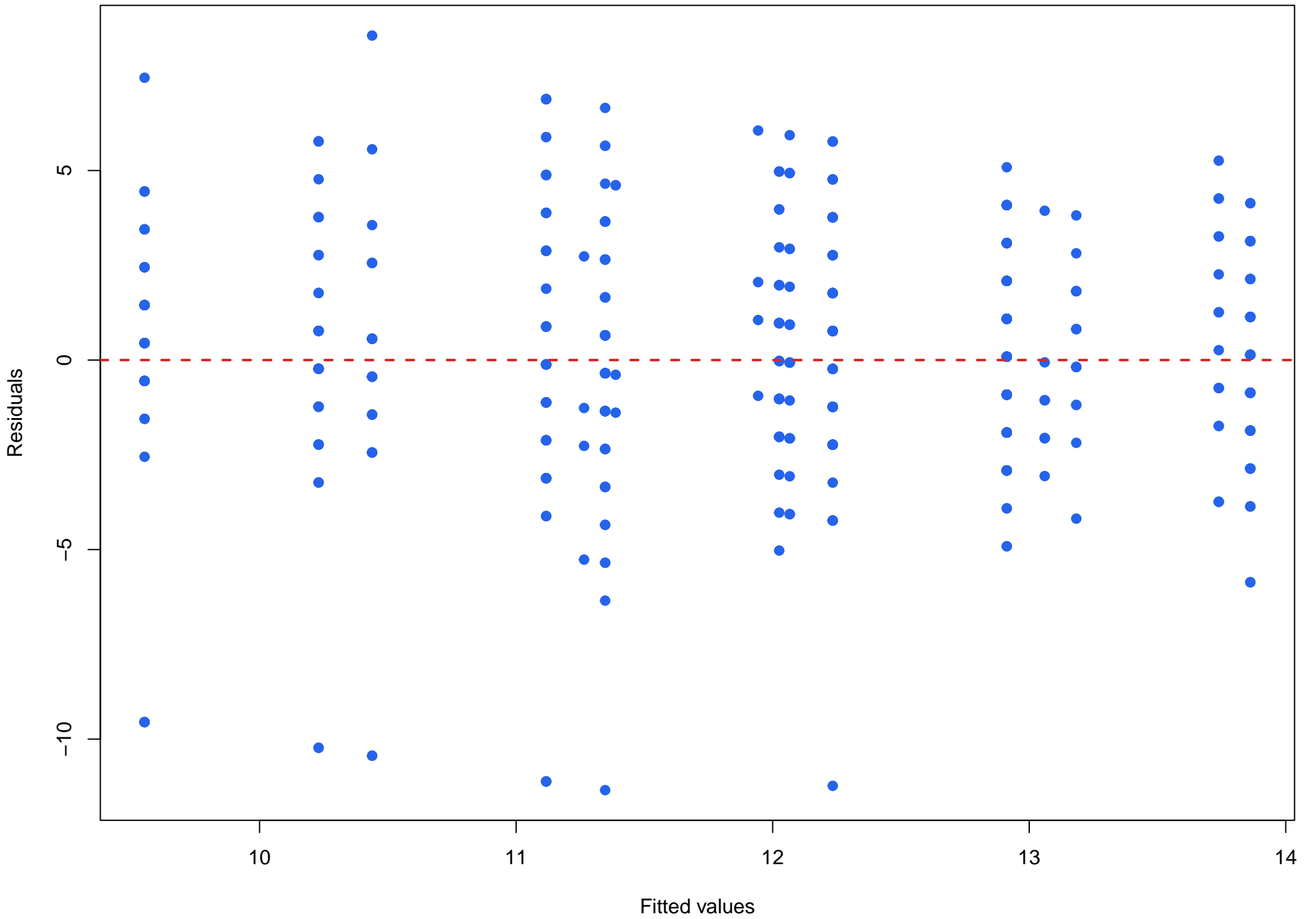
GLM ANOVA: Residuals vs Fitted
